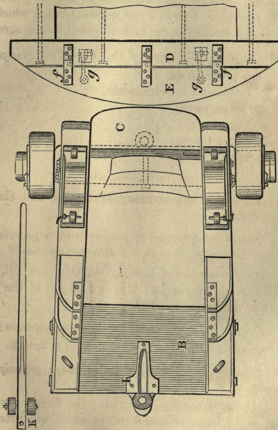
Marsilly Carriage for IX-Inch Shell Gun. Fig. 2.
